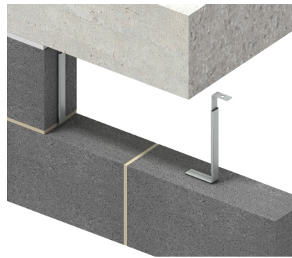
Ancon IHR-B with 9mm dia. hole
