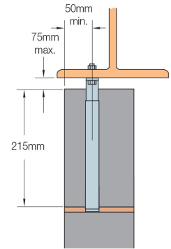
Ancon IHR-C to suit cast-in channel
