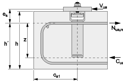
FIGURE 5—ANCHOR REINFORCEMENT TO RESIST SHEAR LOADS
