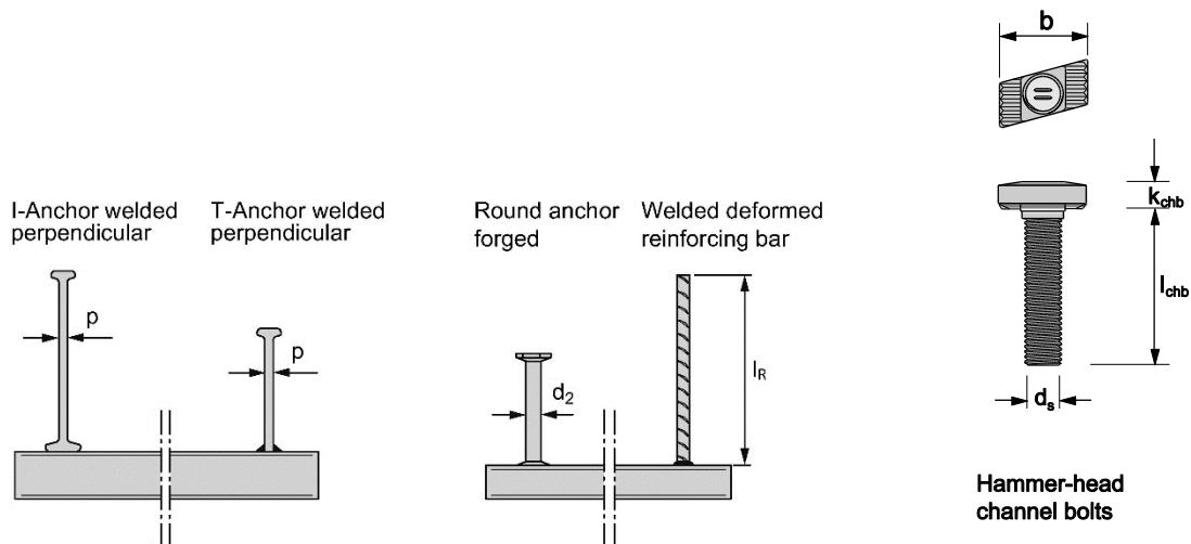
FIGURE B— I- AND T-ANCHORS, ROUND ANCHORS AND DEFORMED REINFORCING BARS FIGURE C—CHANNEL BOLTS
