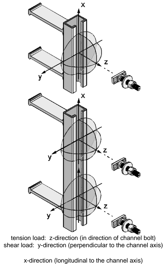
FIGURE 1—LOAD DIRECTIONS
