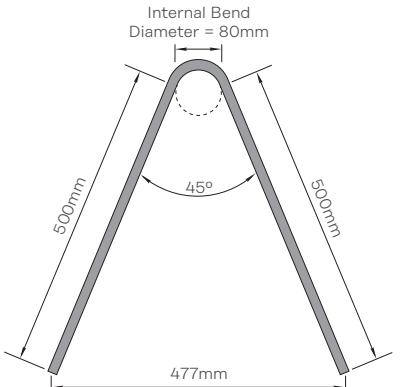
Recommended HD16 or HD20 Tension Bar Diagram 1
