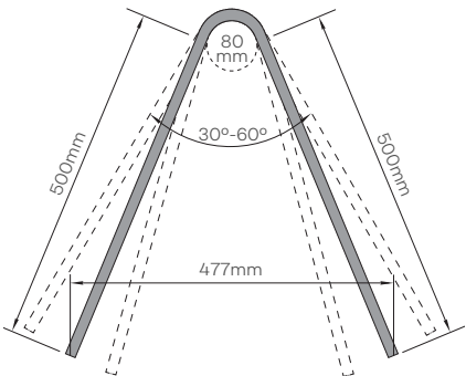
HD16 or HD20 Tension Bar Variations Diagram 2
